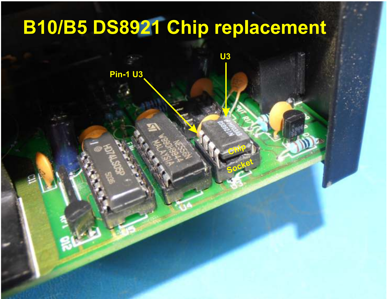
B10/B5 Component Side
